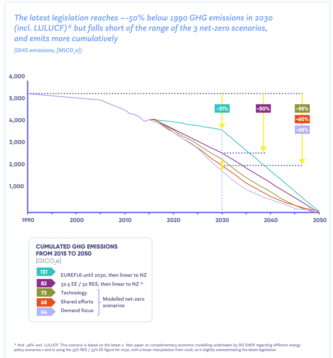
FIGURE 15. Required emissions reduction effort between 2030 and 2050 under various net-zero scenarios
